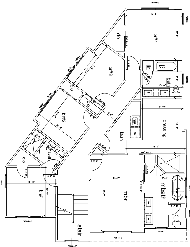
2ND FLOOR AREA 1,591 SF
